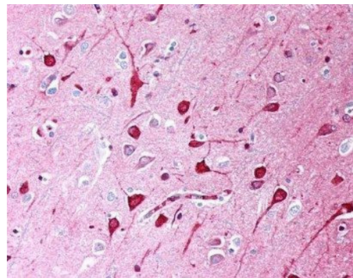
TGF beta-1 Antibody (MA5-16949) in IHC (P) Immunohistochemical staining of human brain showing labelling of neurons using a TGF BETA monoclonal antibody (Product # MA5-16949)
