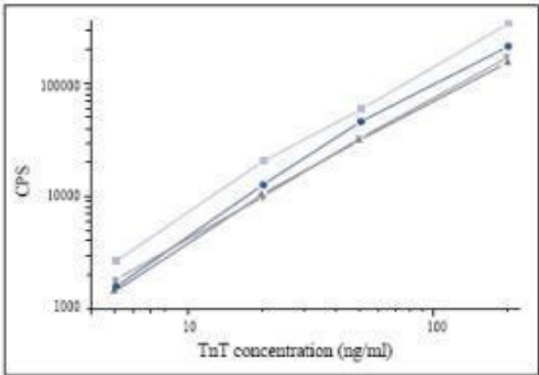
Cardiac Troponin T Antibody (MA1-20879) in ELISA ELISA calibration curves for sandwich cTnT fluoroimmunoassay with different animal TnTs as antigen. (dark blue) canine, (blue/grey) human, (grey) mouse, (black) rat. Monoclonal antibodies: Capture, Cardiac Troponin T Monoclonal Antibody (clone 1C11), 1 g/well. Detection: Cardiac Troponin T Monoclonal Antibody (7E7) (Product # MA1-20879).
