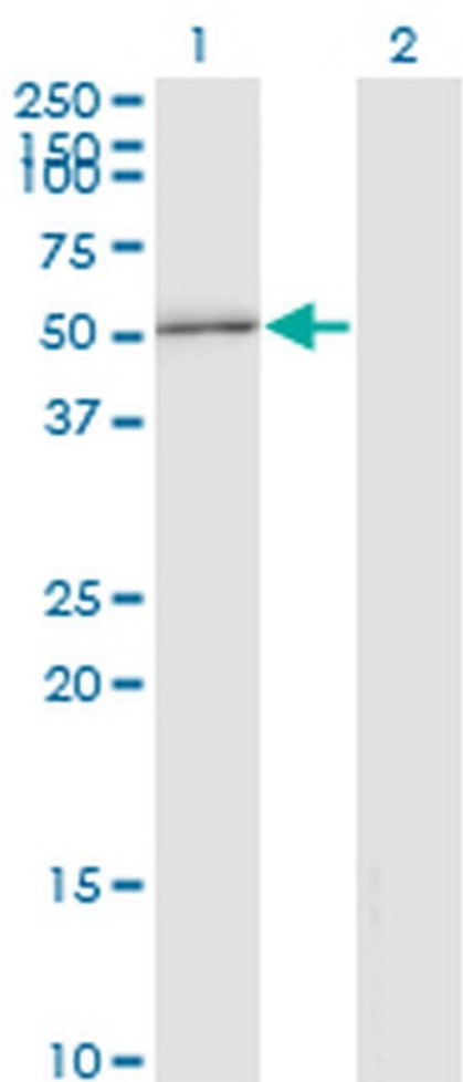
STAU2 Antibody (MA5-21686) in WB Western Blot analysis of STAU2 expressed in transfected 293T cell line by anti-STAU2 monoclonal antibody (Product # MA5-21686), clone 3B7. Lane 1: STAU2 transfected lysate (Predicted MW: 52.8 KDa). Lane 2: Non-transfected lysate.
