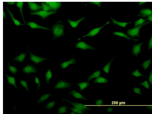
STAU2 Antibody (MA5-21686) in ICC/IF Immunofluorescence analysis of HeLa cells using an anti-STAU2 monoclonal antibody (Product # MA5-21686). (antibody concentration 15 μg/mL).
