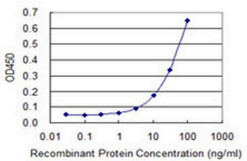
C20orf10 Antibody (MA5-21720) in ELISA Detection limit for recombinant GST tagged TP53TG5 using anti-TP53TG5 monoclonal antibody (Product # MA5-21720) is 1 ng/mL as a capture antibody.
