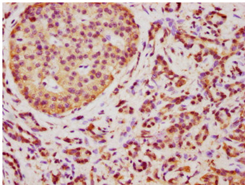
TMEM14A Antibody (PA5-112745) in IHC (P) Immunocytochemical analysis of paraffin-embedded TMEM14A in human pancreatic cancer using a TMEM14A Polyclonal antibody (Product # PA5-112745) at a dilution of 1:350.
