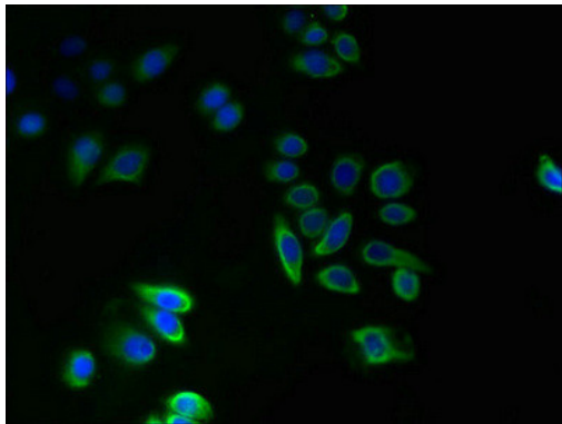
TMEM14A Antibody (PA5-112745) in ICC/IF Immunocytochemical analysis of TMEM14A in PC-3 cells using a Polyclonal antibody (Product # PA5-112745) at a dilution of 1:100. An Alexa Fluor 488-conjugated Goat Anti-Rabbit IgG(H+L) secondary antibody was used.
