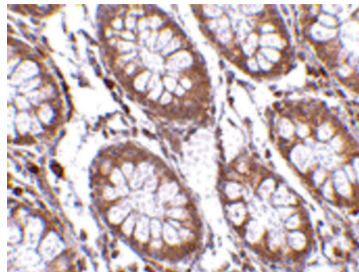
PTK7 Antibody (PA5-20424) in IHC Immunohistochemistry of PTK7 in human colon tissue with PTK7 Polyclonal Antibody (Product # PA5-20424) at 2.5 µg/mL.
