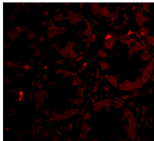
PTK7 Antibody (PA5-20424) in ICC/IF Immunofluorescence of PTK7 in Human Colon cells with PTK7 Polyclonal Antibody (Product # PA5-20424) at 20 µg/mL.
