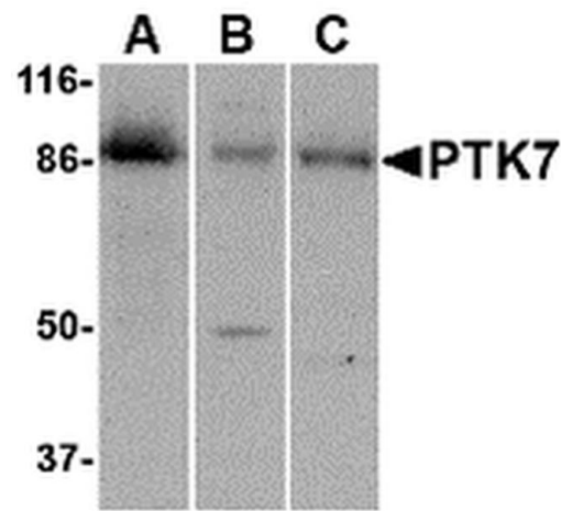
PTK7 Antibody (PA5-20424) in WB Western Blot analysis of PTK7 in (A) human colon, (B) mouse kidney and (C) rat liver tissue lysate with PTK7 Polyclonal Antibody (Product # PA5-20424) at 1 µg /mL.
