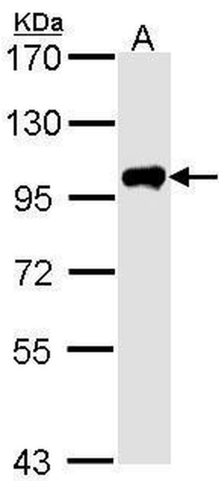
Calpain 3 Antibody (PA5-27721) in WB Western Blot using Calpain 3 Polyclonal Antibody (Product # PA5-27721). Sample (30 µg of whole cell lysate). Lane A: Hela . 7.5% SDS PAGE. Calpain 3 antibody . Calpain 3 Polyclonal Antibody (Product # PA5-27721) diluted at 1: 1,000.
