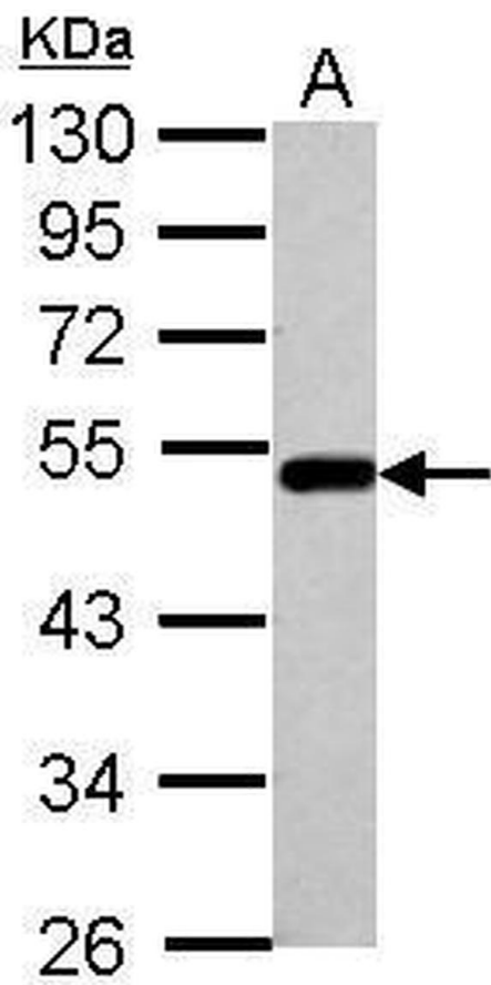
BLMH Antibody (PA5-34680) in WB Western Blot using BLMH Polyclonal Antibody (Product # PA5-34680). Sample (30 µg of whole cell lysate). Lane A: A549. 10% SDS PAGE. BLMH Polyclonal Antibody (Product # PA5-34680) diluted at 1:1,000.
