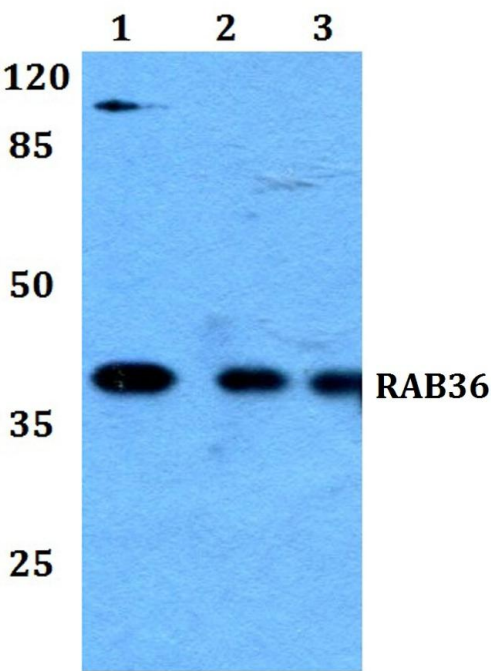
RAB36 Antibody (PA5-37207) in WB Western blot analysis of RAB36 in Lane 1: HEK293T whole cell lysate, Lane 2: NIH-3T3 whole cell lysate, Lane 3: PC12 whole cell lysate. Samples were incubated with RAB36 polyclonal antibody (Product # PA5-37207) at a dilution of 1:500.
