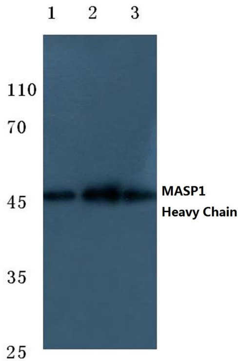
MASP1 Antibody (PA5-37428) in WB Western blot analysis of MASP1 in Lane 1: A549 cell lysate treated with colchicine, Lane 2: mouse lung tissue lysate, Lane 3: rat liver tissue lysate. Samples were incubated with MASP1 polyclonal antibody (Product # PA5-37428) at a dilution of 1:500.
