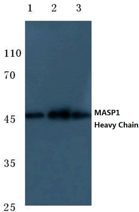
MASP1 Antibody (PA5-37428) in WB Western blot analysis of MASP1 using MASP1 polyclonal antibody (Product # PA5-37428) at a dilution of 1:500. Lane 1: A549 cell lysate treated with colchicine, Lane 2: Mouse lung tissue lysate, Lane 3: Rat liver tissue lysate.
