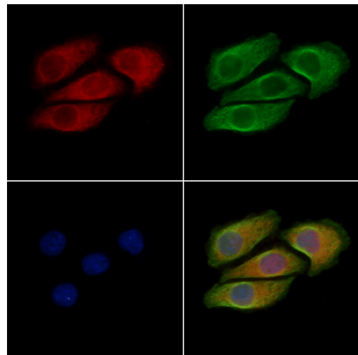
Phospho-B-Raf (Thr599) Antibody (PA5-37497) in ICC/IF Immunocytochemical analysis of Phospho-B-Raf (Thr599) in methanol-fixed Hela cells, using Phospho-B-Raf (Thr599) Polyclonal Antibody (Product # PA5-37497).
