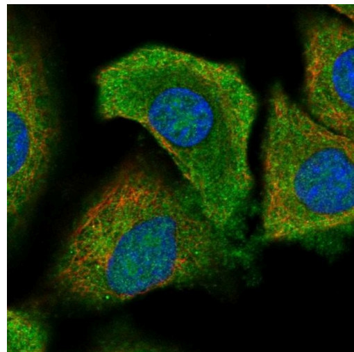
WDFY3 Antibody (PA5-61771) in ICC/IF Immunofluorescent staining of WDFY3 in human cell line A549 using a WDFY3 Polyclonal Antibody (Product # PA5-61771) shows localization to nucleoli and cytosol.
