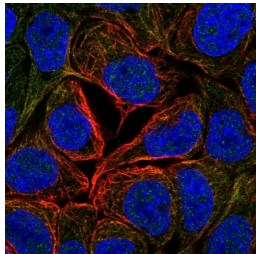
GAN Antibody (PA5-61982) in ICC/IF Immunofluorescent staining of GAN in human cell line RT4 using a GAN Polyclonal Antibody (Product # PA5-61982) shows localization to microtubules.
