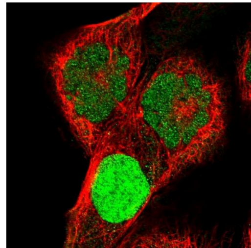
KV4.1 (KCND1) Antibody (PA5-64866) in ICC/IF Immunofluorescent staining of KCND1 in human cell line A-431 shows localization to nucleus. Samples were probed using a KCND1 Polyclonal Antibody (Product # PA5-64866).
