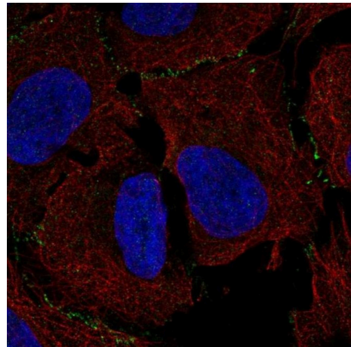
MAGI3 Antibody (PA5-64925) in ICC/IF Immunofluorescent staining of MAGI3 in human cell line U-2 OS shows localization to cell junctions. Samples were probed using a MAGI3 Polyclonal Antibody (Product # PA5-64925).
