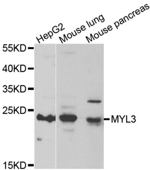
MYL3 Antibody (PA5-76981) in WB Western blot analysis of MYL3. Samples were incubated with MYL3 polyclonal antibody (Product # PA5-76981).
