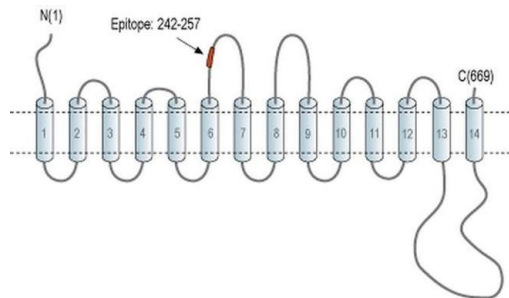
SGLT2 (extracellular) Antibody (PA5-77461) (C)KDPVAVGNISST(S)YQPR, corresponding to amino acid residues 242-257 of rat SGLT2
