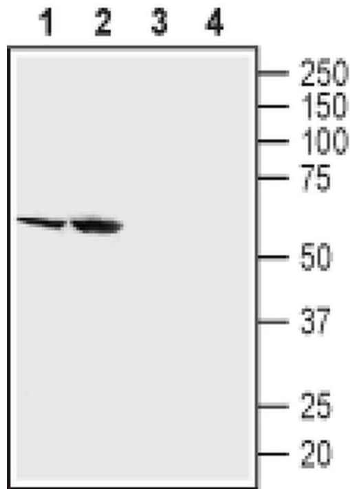
SGLT2 (extracellular) Antibody (PA5-77461) in WB Western blot analysis of mouse kidney lysates (lanes 1 and 3) and rat kidney membranes (lanes 2 and 4) with SGLT2 (extracellular) polyclonal antibody (Product # PA5-77461) using a dilution of 1:200.
