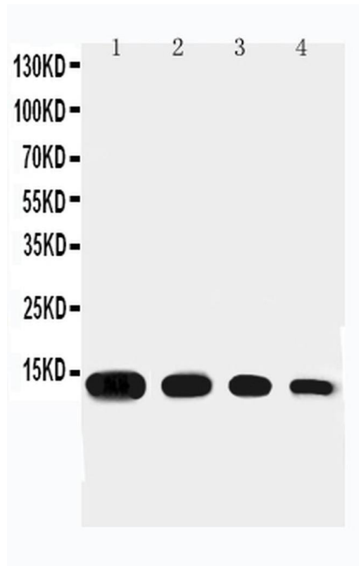
Eotaxin Antibody (PA5-78930) in WB Western blot analysis of Eotaxin in Lane 1: recombinant mouse Eotaxin protein, Lane 2: recombinant mouse Eotaxin protein, Lane 3: recombinant mouse Eotaxin protein, Lane 4: recombinant mouse Eotaxin protein 1.25 ng using 10, 5 and 2.5 ng, respectively per well. Sample was incubated with Eotaxin (Product # PA5-78930).
