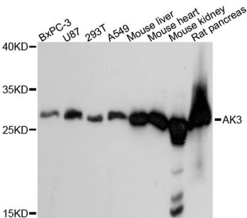
Adenylate Kinase 3 Antibody (PA5-87137) in WB Western blot analysis of Adenylate Kinase 3 in various cell lines. Sample was incubated with Adenylate Kinase 3 polyclonal antibody (Product # PA5-87137) using a 1:3000 dilution.
